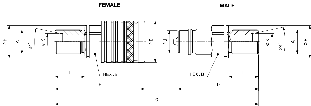
Port description: MALE THREAD METRIC L SCHOTT – BULKHEAD SERIES – 24°CONE (ISO 8434-1 & DIN 2353)
